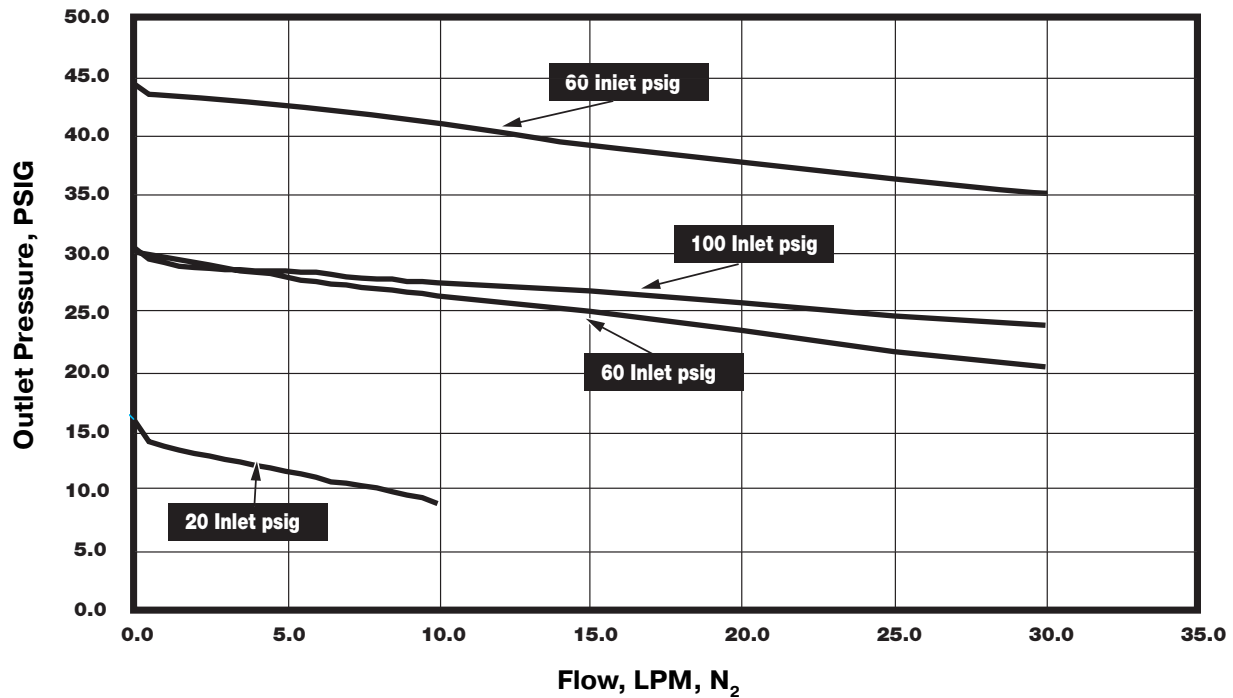
SMSQ2Micro 1-1/8" Flow Curve
